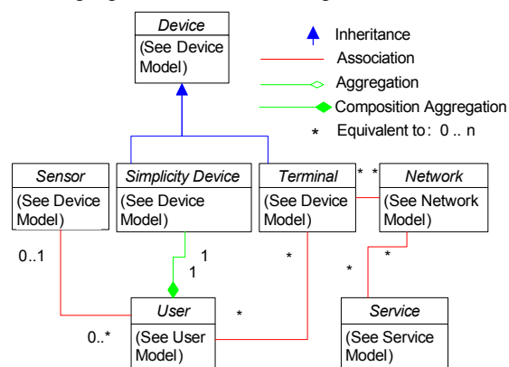
Figure 2: Core model of the information model
