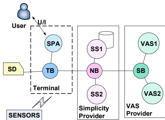
Figure 1: Simplicity architecture
